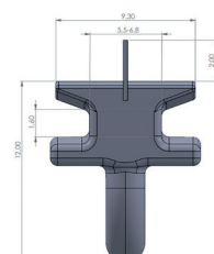
Glider Tape - 6mm inner track - Fixed eyelet
