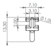
Glider Cord - 4mm inner track - Fixed Eyelet
